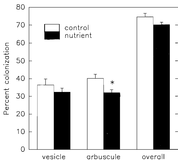
FIG. 1. Percent colonization of vesicles, arbuscules, and overall VAM infection in Agropyron desertorum . The vertical bars represent the standard error of each mean ( n = 20 ) averaged over date, depth, and treatment. The asterisk indicates statistical significance with p = 0.03 .
